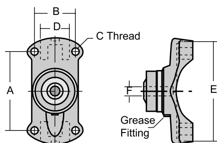
Type 1 (Greaseable)
