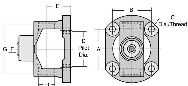
Type 2 (Non-Greaseable)
