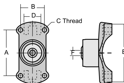
Type 2 (Non-Greaseable)
