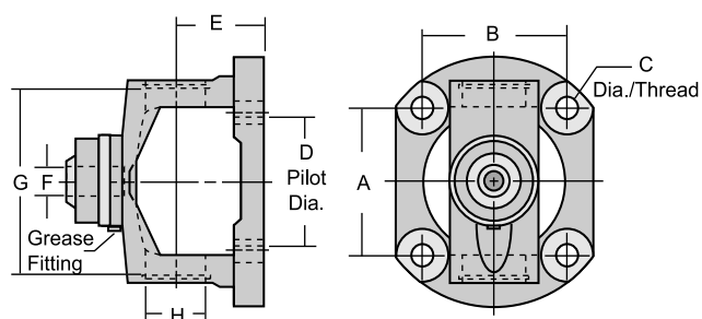
Type 1 (Greaseable)
